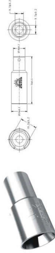
TBulkhead wrench tool: P/N for M12: H4TM1200; P/N for M14: H4TM1400
