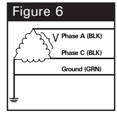
Figure 6 CORNER GROUND DELTA (B grounded) 2 Hots, 1 Grnd
