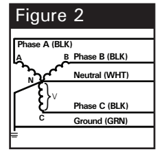
Figure 2 WYE 3 Hots, 1 Neu, 1 Grnd
