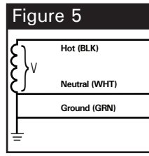
Figure 5 SINGLE POLE 1 Hot, 1 Neu, 1 Grnd
