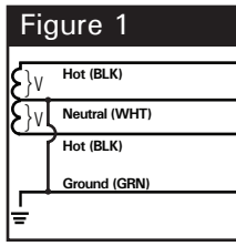
Figure 1 SPLIT 2 Hots, 1 Neu, 1 Grnd
