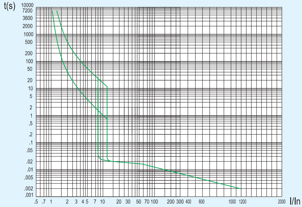
NM8-125(80A,100A)
