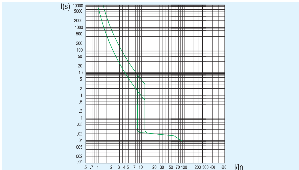
NM8-800, 1250(800A~1250A)
