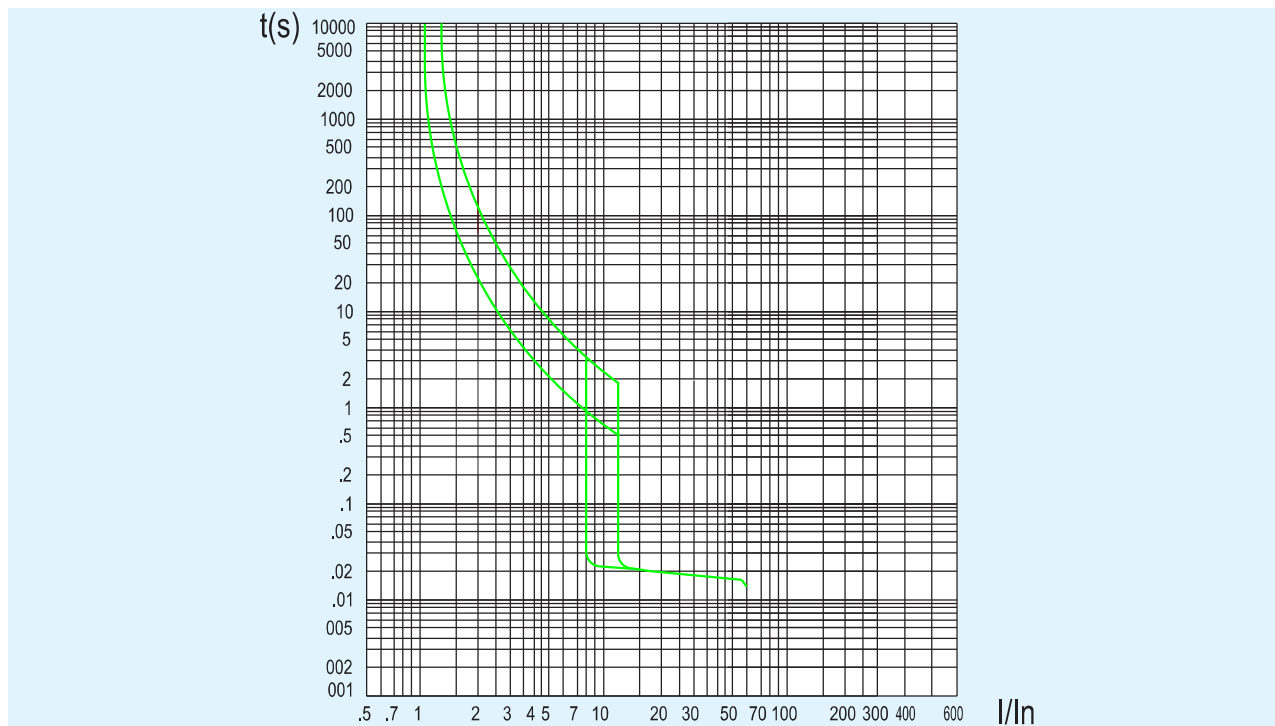
NM8-800, 1250(800A~1250A)
